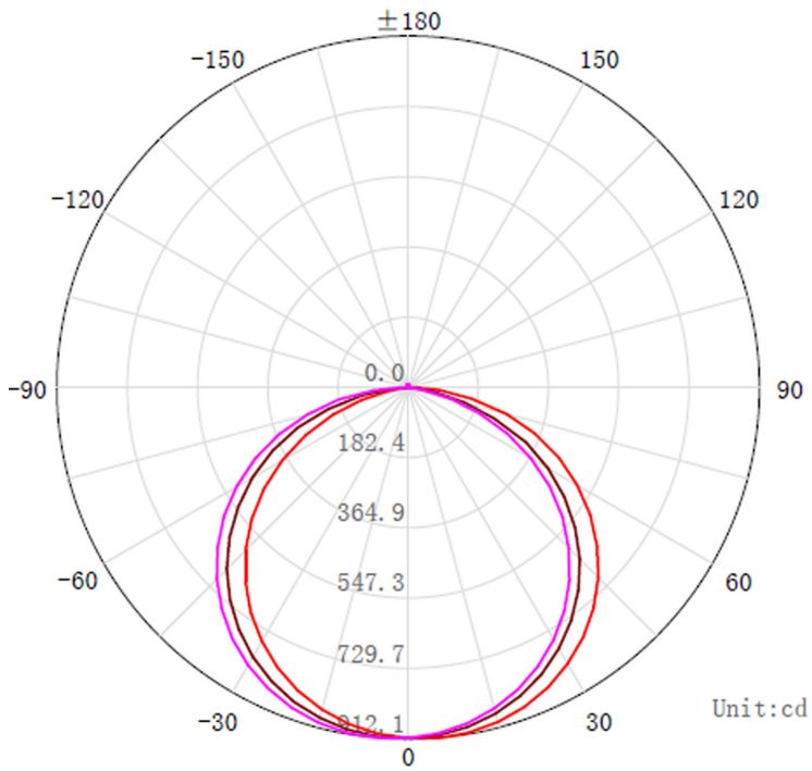
C Plane Distribution Diagram
